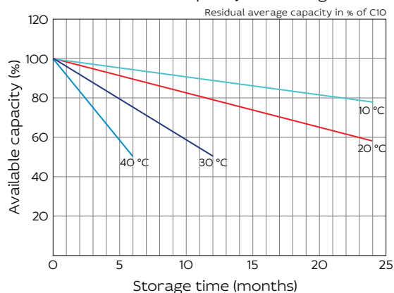
General Relation of Capacity VS. Storage Time
