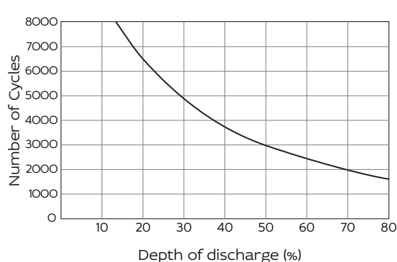
Cycle Life in Relation to DOD
